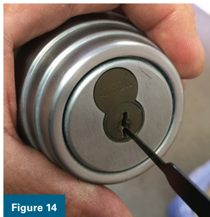
Figures 13-15. To remove a small format IC core intact, get to the back of the core (Figure 13), put pressure on the locking dog, and try to pick it (Figure 14). The result is shown in Figure 15.
