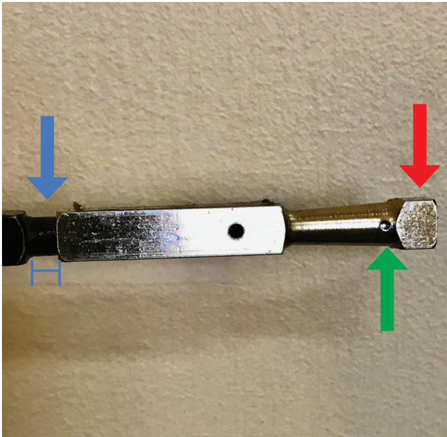
Figure 5. The red arrow is pointing to the approximate spot the set screw bit into. The green arrow points to a bite mark on the taper from the set screw.
